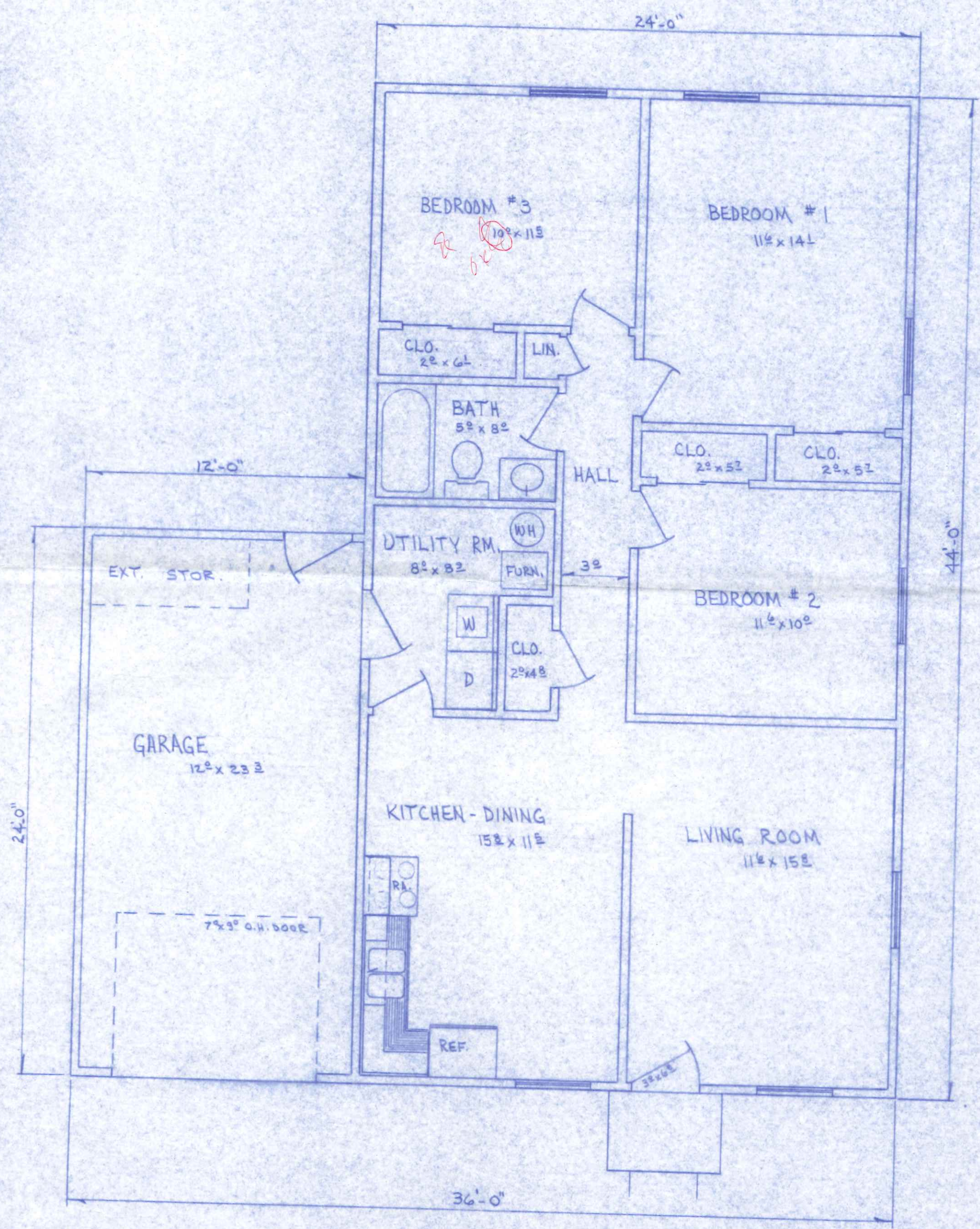
FLOOR PLAN 1/4" = 1'-0"
