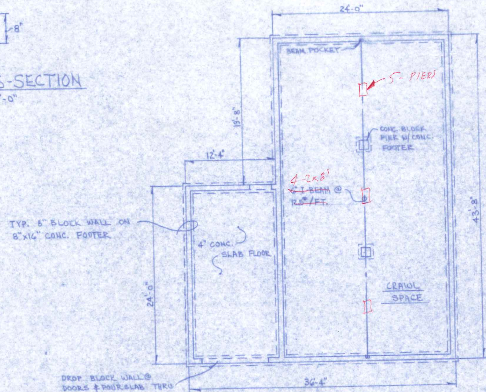
FOUNDATION PLAN 1/8" = 1'-0"
