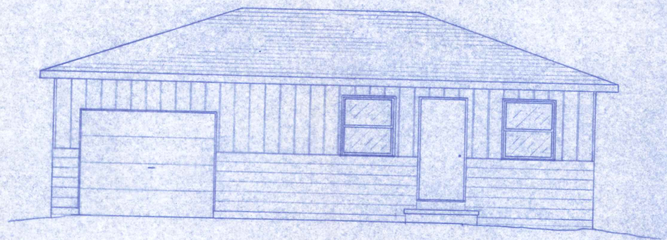
FRONT ELEVATION 1/4" = 1'-0"
