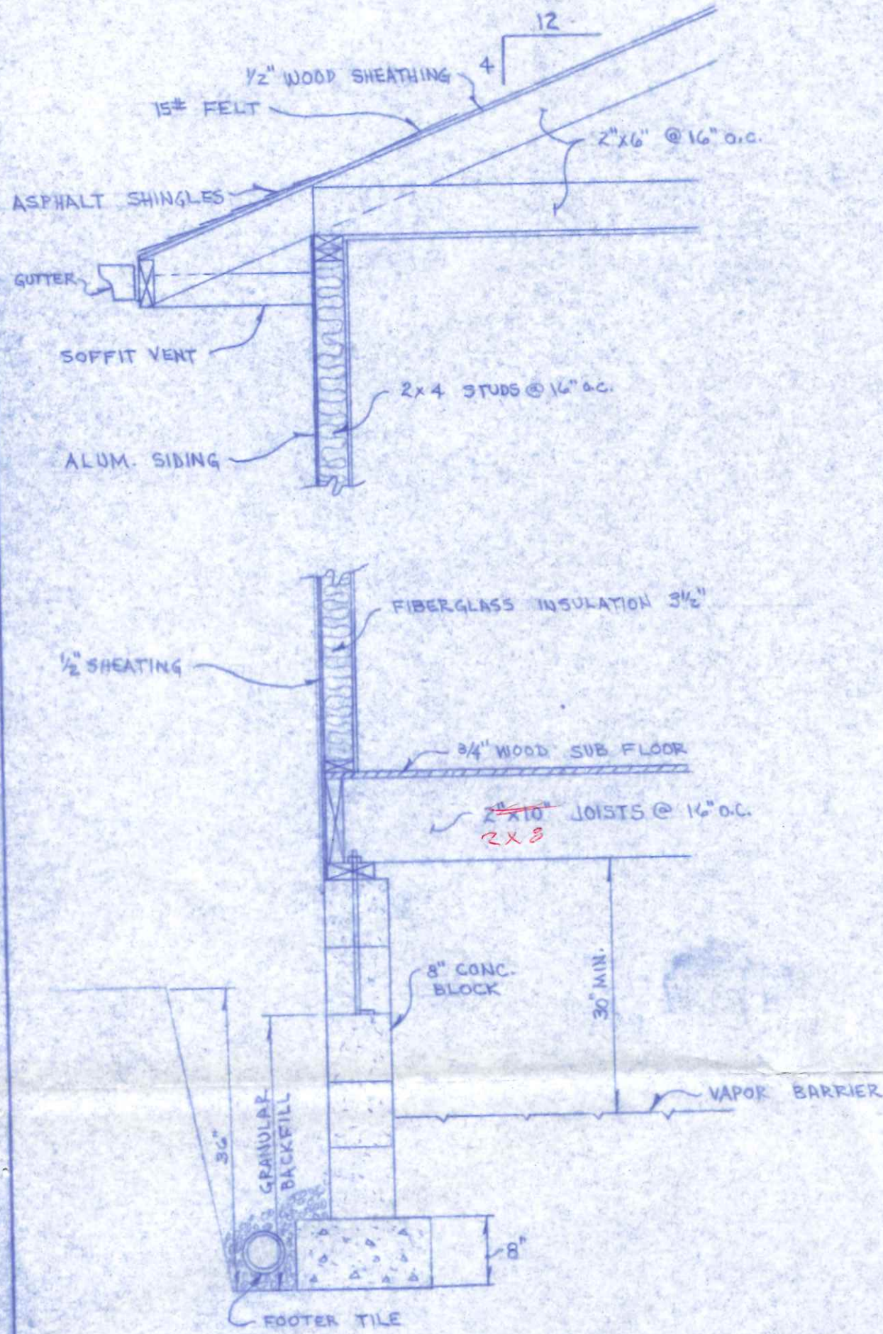
TYPICAL CROSS-SECTION 3/4" = 1'-0"
