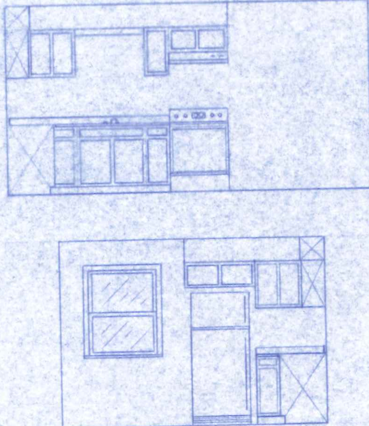
KITCHEN DETAILS 1/4" = 1'-0"
